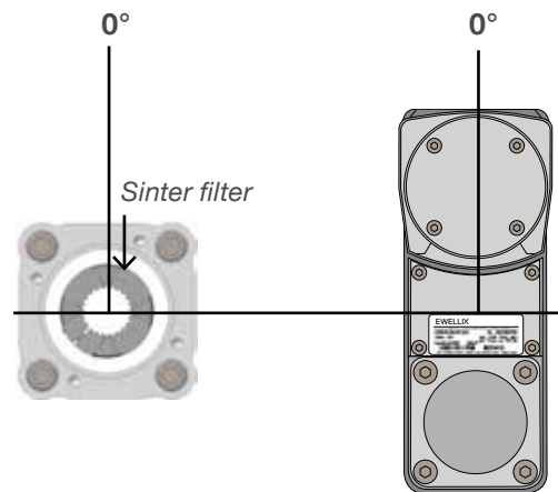
Gearbox reference
